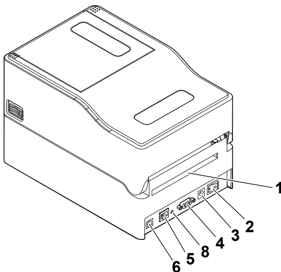
Standard model
