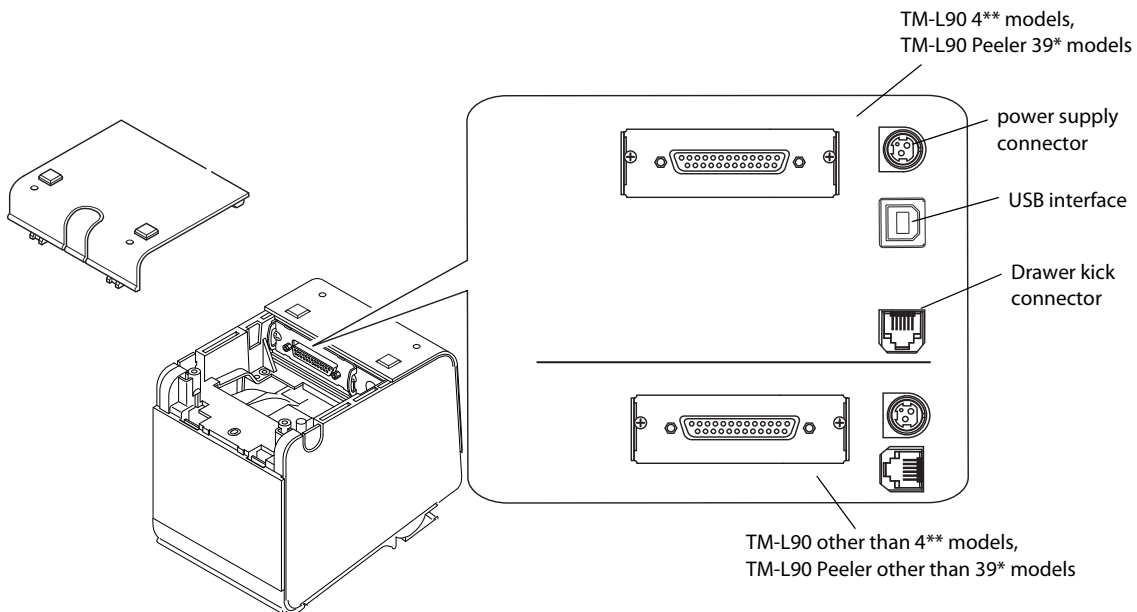
Connector Panel
