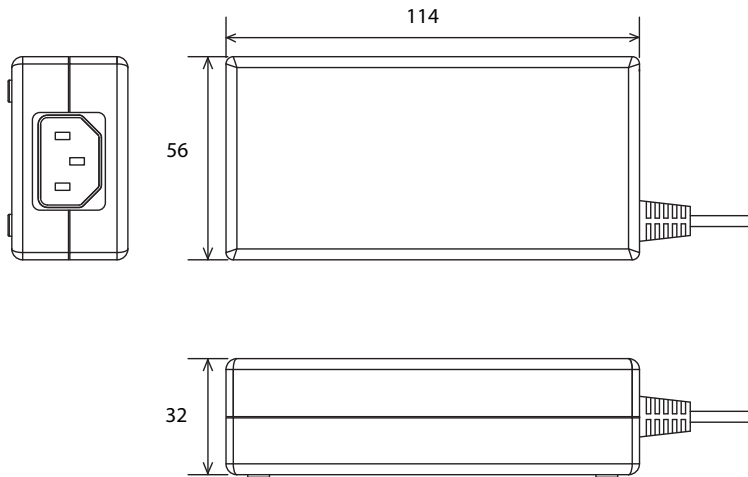
Case specifications
